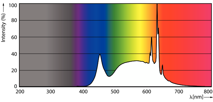
Spectral Power Distribution Colour - 12.2A19/COR/940/FR/P/E26/DIM/T20 6/1CT
