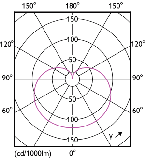
Light Distribution Diagram - 12.2A19/COR/940/FR/P/E26/DIM/T20 6/1CT
