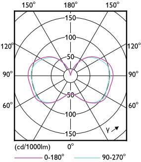
Light Distribution Diagram - 18CC/LED/850/ND E26 G2 BB 6/1
