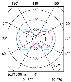
Light Distribution Diagram - 27CC/LED/850/ND E26 G2 BB 6/1
