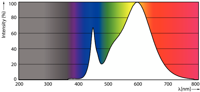
Spectral Power Distribution Colour - 36CC/LED/830/ND E26 G2 BB 6/1
