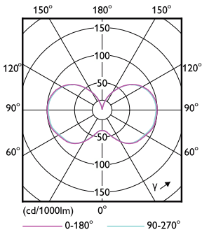
Light Distribution Diagram - 36CC/LED/850/ND E26 G2 BB 6/1
