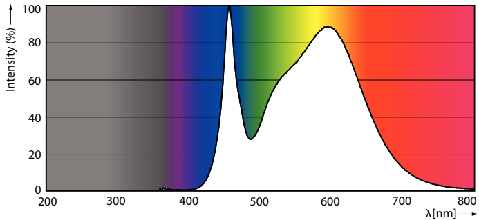
Spectral Power Distribution Colour – TForce Core HB MV ND 35W E27 840 G3
