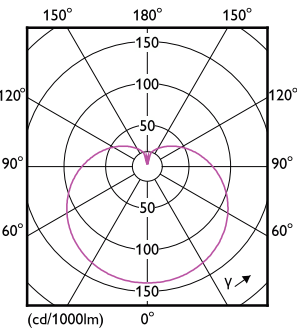
Light Distribution Diagram - LEDGlobe 10-75W G120 E27 WW 230V_AU
