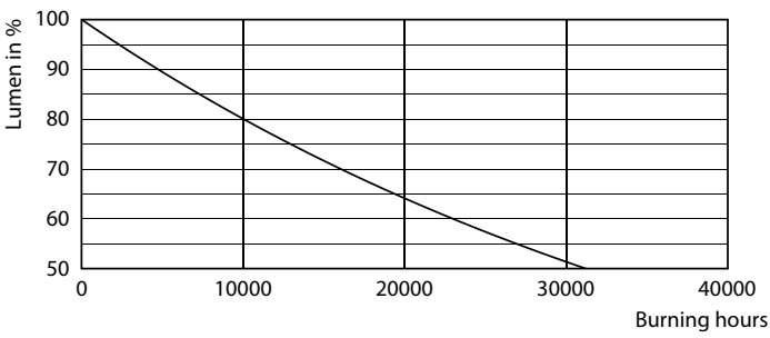
Lumen Maintenance Diagram - CorePro LED spot ND 2.9-20W MR16 827 36D
