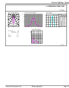
Accent Lighting Spots - CorePro LED spot ND 2.9-20W MR16 827 36D
