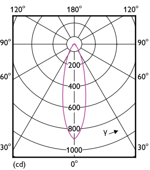
Light Distribution Diagram - CorePro LED spot ND 4.4-35W MR16 840 36D
