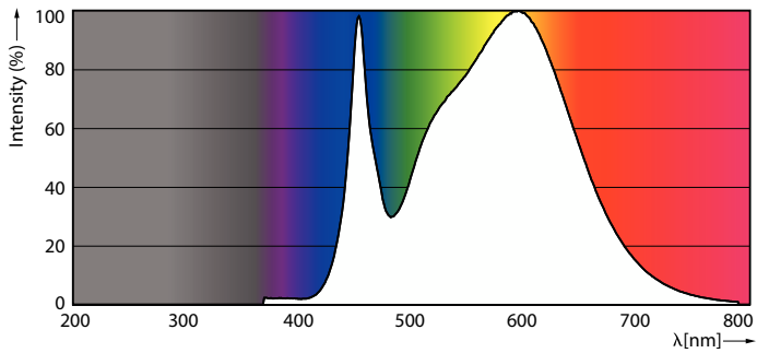
Spectral Power Distribution Colour - 145HB/MAS/840/D NB DL BB G2 4/1
