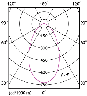
Light Distribution Diagram - 145HB/MAS/840/D NB DL BB G2 4/1
