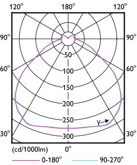
Light Distribution Diagram - 145HB/LED/840/D WB UDL BB G2 4/1
