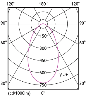
Light Distribution Diagram - 145HB/MAS/850/D NB DL BB G2 4/1
