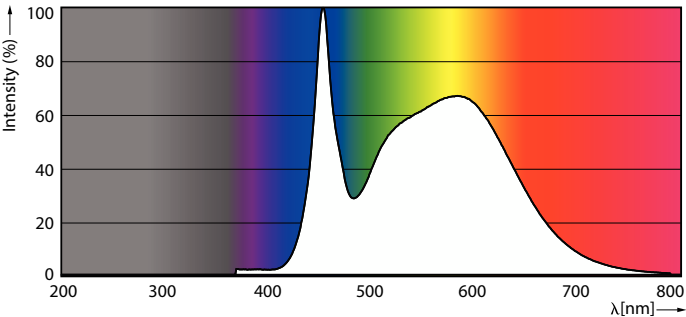
Spectral Power Distribution Colour - 145HB/MAS/850/D NB DL BB G2 4/1
