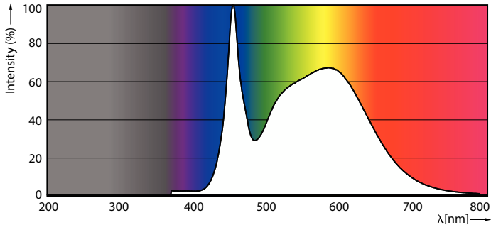
Spectral Power Distribution Colour - 145HB/LED/850/D WB UDL BB G2 4/1
