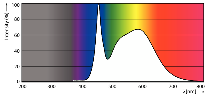
Spectral Power Distribution Colour - 145HB/MAS/850/D WB UDL BB G2 4/1
