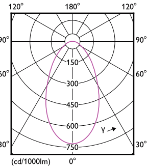
Light Distribution Diagram - 165HB/MAS/840/D NB DL BB G2 4/1
