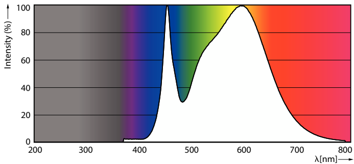
Spectral Power Distribution Colour - 165HB/MAS/840/D NB DL BB G2 4/1
