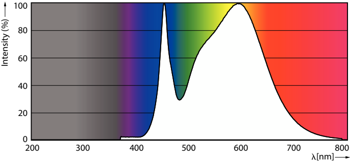
Spectral Power Distribution Colour - 165HB/MAS/840/D WB UDL BB G2 4/1
