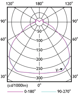
Light Distribution Diagram - 165HB/MAS/840/D WB UDL BB G2 4/1
