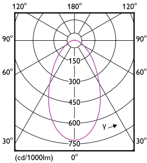
Light Distribution Diagram - 165HB/MAS/850/D NB DL BB G2 4/1
