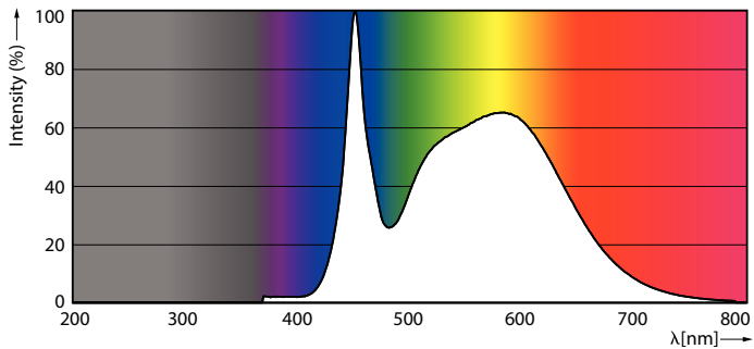
Spectral Power Distribution Colour - 165HB/MAS/850/D NB DL BB G2 4/1
