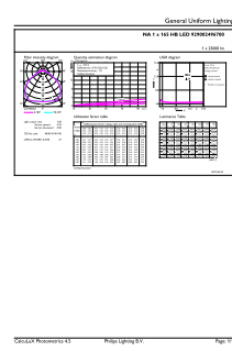
General uniform lighting - 165HB/MAS/850/D WB UDL BB G2 4/1
