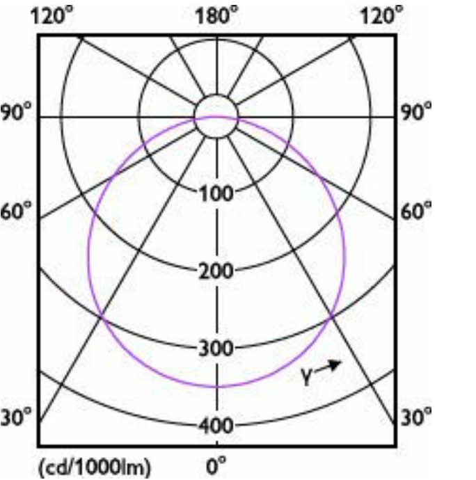
Light Distribution Diagram - DL252 G2 SF RD LED 2000 65K 24W 11" WW
