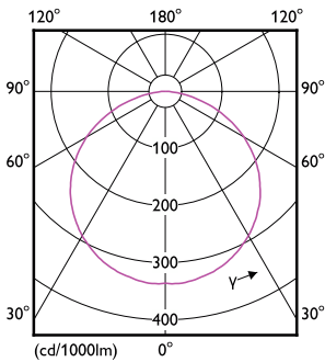
Light Distribution Diagram - MAS LEDstrip 16.6W940 2000LM/M 5M
