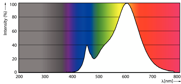
Spectral Power Distribution Colour - LEDLuster 5W P45 2700K E27 ND FR AU 2CT
