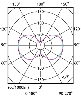
Light Distribution Diagram - 36CC/LED/830/LS EX39 G3 BB 3/1
