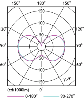
Light Distribution Diagram - 36CC/LED/840/LS EX39 G3 BB 3/1
