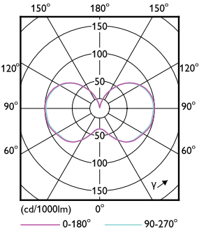
Light Distribution Diagram - 36CC/LED/840/LS EX39 G3 BB 3/1
