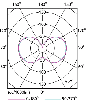
Light Distribution Diagram - 36CC/LED/850/LS EX39 G3 BB 3/1
