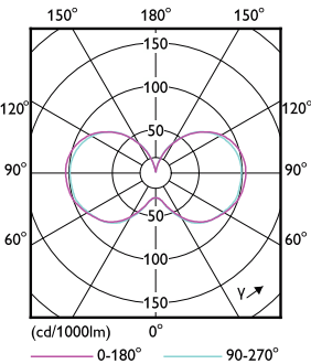
Light Distribution Diagram - 45CC/LED/830/LS EX39 G3 BB 3/1
