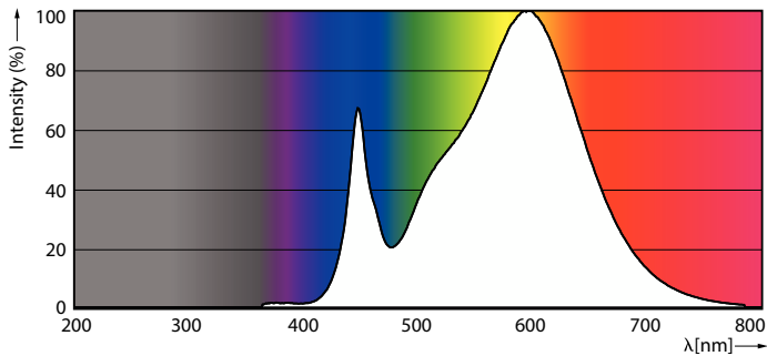
Spectral Power Distribution Colour - 45CC/LED/830/LS EX39 G3 BB 3/1
