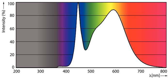
Spectral Power Distribution Colour - 54CC/LED/840/LS EX39 G3 BB 3/1
