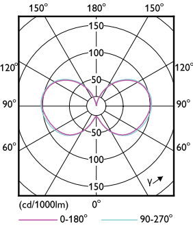
Light Distribution Diagram - 63CC/LED/840/LS EX39 G3 BB 3/1
