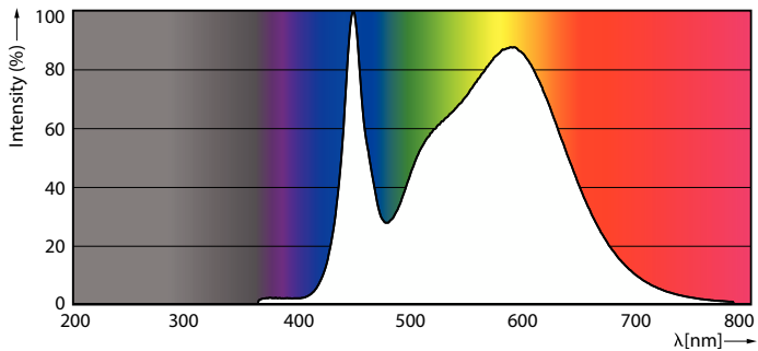
Spectral Power Distribution Colour - 63CC/LED/840/LS EX39 G3 BB 3/1
