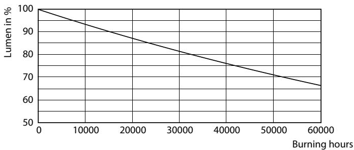
Lumen Maintenance Diagram - 63CC/LED/840/LS EX39 G3 BB 3/1
