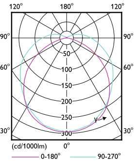
Light Distribution Diagram - 40WP/LED/850/LS EX39 G3 BB 3/1
