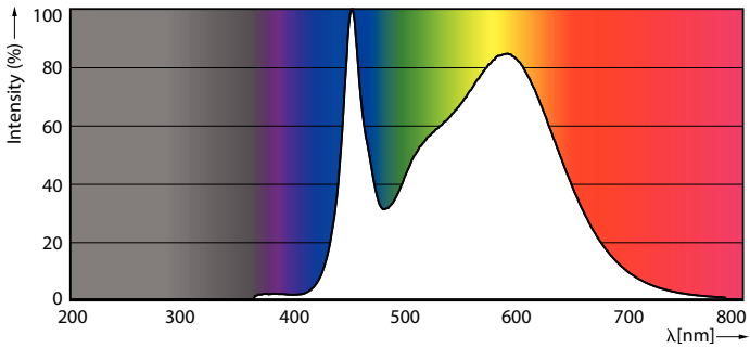
Spectral Power Distribution Colour - 60WP/LED/840/LS EX39 G3 BB 3/1
