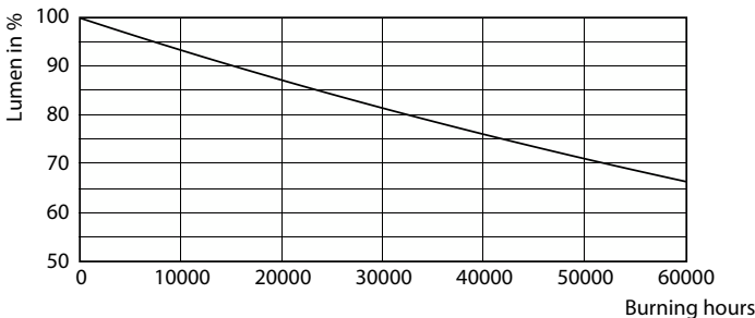
Lumen Maintenance Diagram - 60WP/LED/840/LS EX39 G3 BB 3/1
