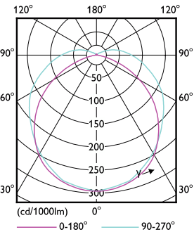
Light Distribution Diagram - 60WP/LED/840/LS EX39 G3 BB 3/1
