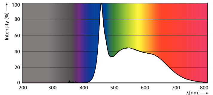
Spectral Power Distribution Colour - LEDBulb 6W E27 965 230V 1PF/6 AU
