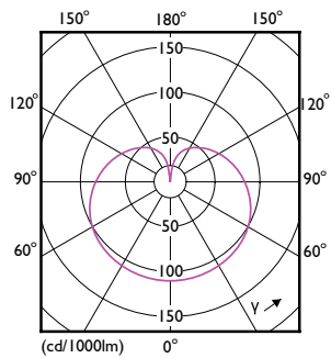
Light Distribution Diagram - LEDBulb 6W B22 965 230V 1PF/6 AU
