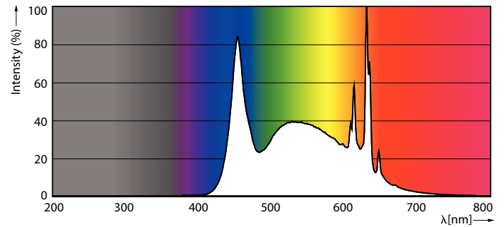
Spectral Power Distribution Colour - LEDBulb 6W B22 965 230V 1PF/6 AU
