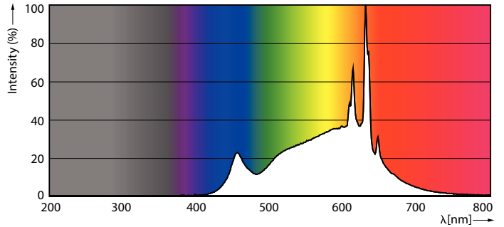
Spectral Power Distribution Colour - LEDBulb 8W B22 930 230V 1PF/6 AU
