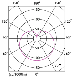
Light Distribution Diagram - LEDBulb 8W B22 930 230V 1PF/6 AU
