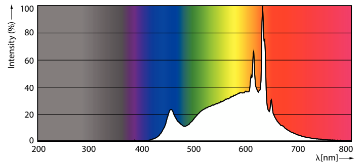
Spectral Power Distribution Colour - LEDBulb 10W B22 930 230V 2PF/3 AU
