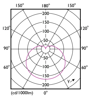
Light Distribution Diagram - LEDBulb 10W B22 930 230V 2PF/3 AU
