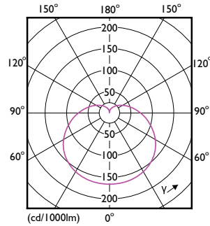
Light Distribution Diagram - LEDBulb 12W B22 930 230V 1PF/6 AU
