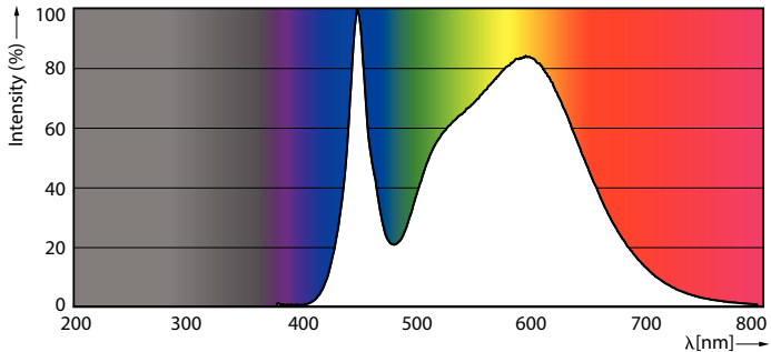
Spectral Power Distribution Colour - 450CC/MAS/840/LS EX39 BB 3/1
