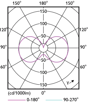
Light Distribution Diagram - 450CC/LED/850/LS EX39 BB 3/1
