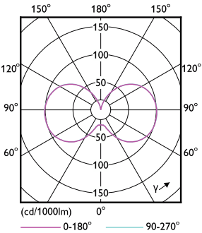
Light Distribution Diagram - 450CC/MAS/850/LS EX39 BB 3/1
