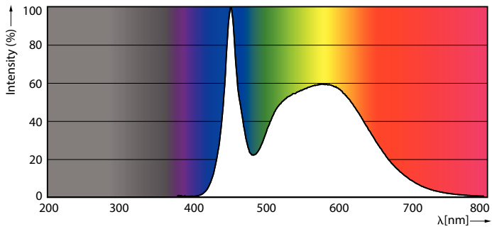
Spectral Power Distribution Colour - 450CC/MAS/850/LS EX39 BB 3/1
