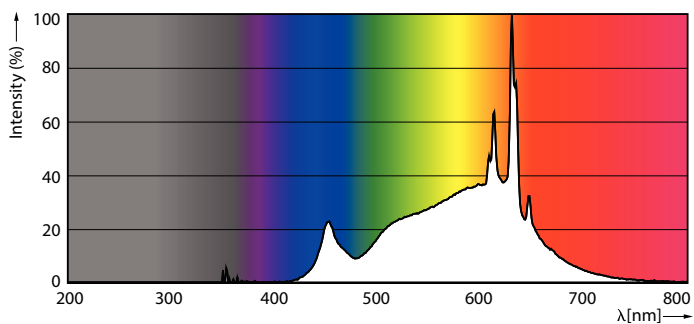
Spectral Power Distribution Colour - 5.5PAR20/LED/F25/930/DIM/G/T20 6/1FB
