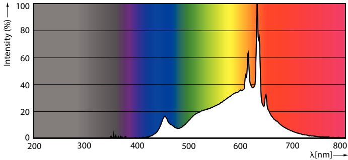
Spectral Power Distribution Colour - 5.5PAR20/LED/F25/927-922/DIM/G/T20 6/1FB
