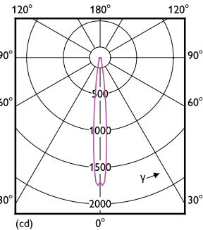
Light Distribution Diagram - MAS ExpertColor 10.8-50W 927 AR111 9D
