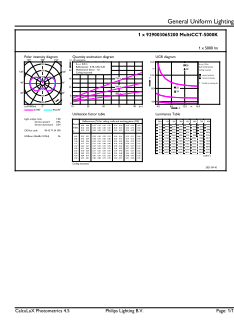
General uniform lighting - 36CC/LED/3CCT/LS EX39 G3 BB 3/1
