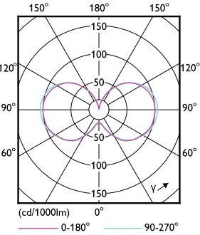
Light Distribution Diagram - 54CC/LED/3CCT/LS EX39 G3 BB 3/1
