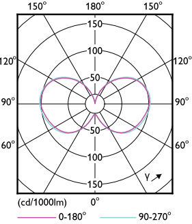
Light Distribution Diagram - 63CC/LED/3CCT/LS EX39 G3 BB 3/1
