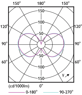
Light Distribution Diagram - 63CC/LED/3CCT/LS EX39 G3 BB 3/1
