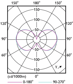
Light Distribution Diagram - 63CC/MAS/3CCT/LS EX39 G3 BB 3/1
