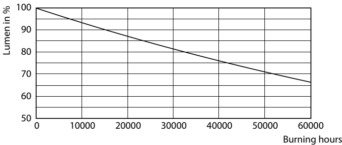
Lumen Maintenance Diagram - 63CC/MAS/3CCT/LS EX39 G3 BB 3/1
