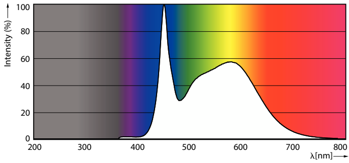
Spectral Power Distribution Colour - 63CC/MAS/3CCT/LS EX39 G3 BB 3/1
