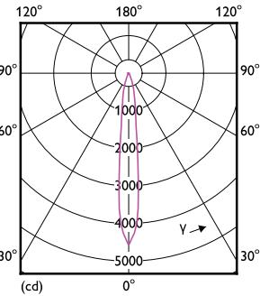
Light Distribution Diagram - MASTER LED 6.5-50W 930 MR16 10D Dim CN
