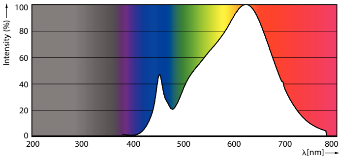
Spectral Power Distribution Colour - MASTER LED 6.5-50W 930 MR16 10D Dim CN
