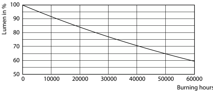
Lumen Maintenance Diagram - MASTER LED 6.5-50W 930 MR16 10D Dim CN
