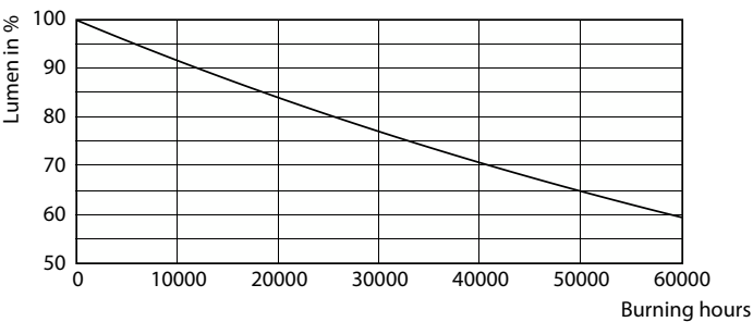
Lumen Maintenance Diagram - MASTER LED 6.5-50W 927 MR16 24D Dim CN
