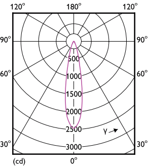
Light Distribution Diagram - MASTER LED 6.5-50W 927 MR16 24D Dim CN
