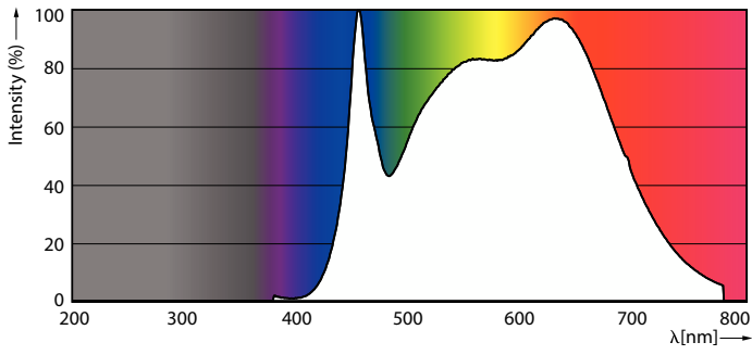
Spectral Power Distribution Colour - 7.8MR16/PER/940/S10/Dim/EC/12V 10/1FB
