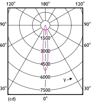
Light Distribution Diagram - 7.8MR16/PER/940/S10/Dim/EC/12V 10/1FB
